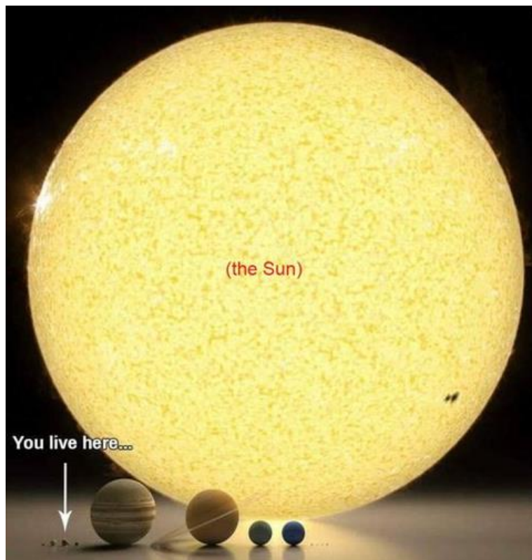
Figure #3 Illustration Of Atum Ur Heka—Our Sun Ra Ur Heka: The Sun—In Ma'at Ur Heka Divine Planetary Order Within Our Milky Way Galaxy.
