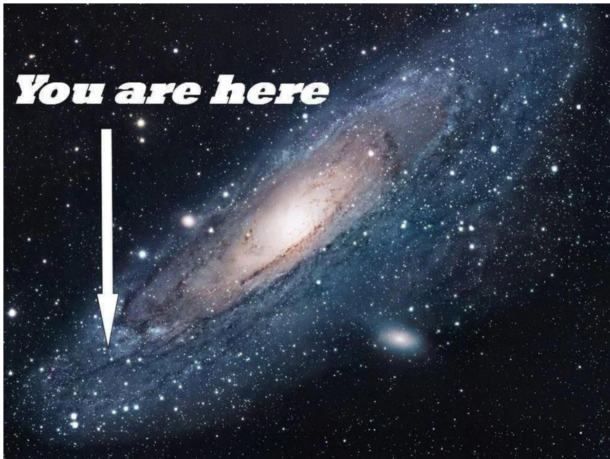
Figure #2 Illustration "You Are Here in Our Milky Way Galaxy."
